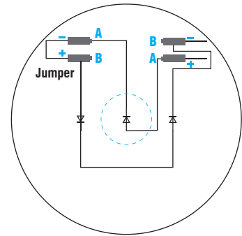
Standard wiring
