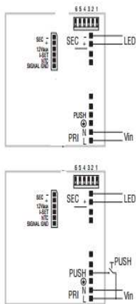
PUSH diagram • Collegamento PUSH
