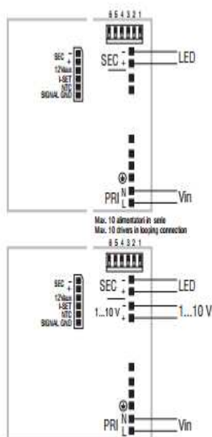
1...10 V diagram • Collegamento 1...10 V
