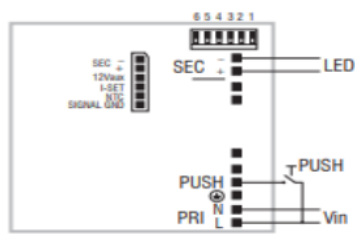
PUSH diagram - Collegamento PUSH
