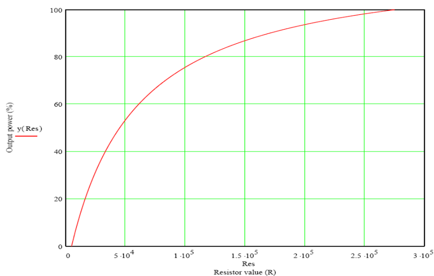
Output power vs Iset resistor (1-10V and Push mode only)
