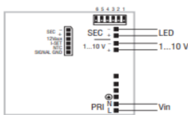
1...10 V diagram - Collegamento 1...10 V
