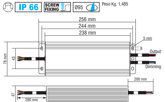
DC 150W VPS 1-10V - DC 180W VPS 1-10V - DC 200W VPS 1-10V
