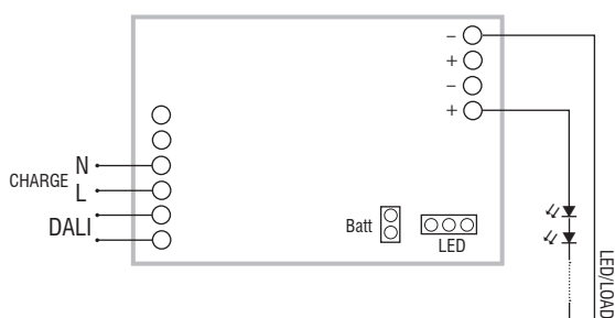
Non-maintained (emergency only) diagram Collegamento non permanente (solo emergenza)
