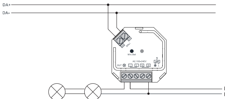
DALI MASTER connection
