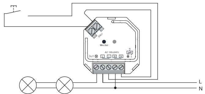
PUSH SWITCH connection
