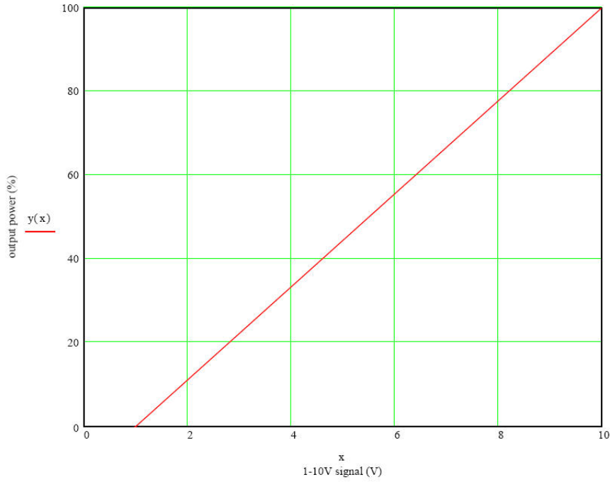
Output power vs 1-10V signal
